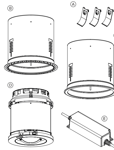
A - Fixing Clips (x3) B - Trimless Mounting Ring C - Standard Mounting Ring D - DRX7 Luminaire E - Power Supply
